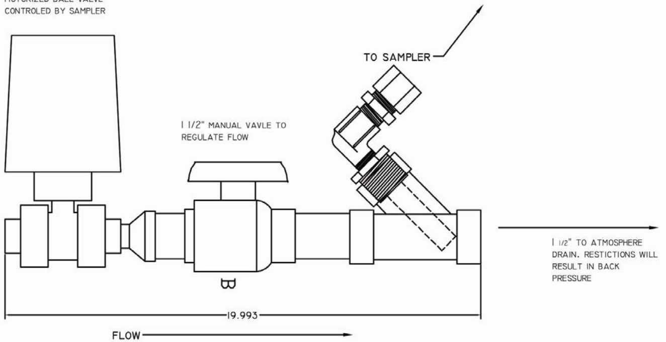
Flow-through Cell High Flow Setup
